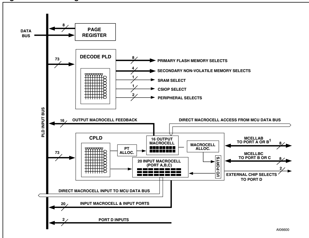
Figure 53. PLD diagram
