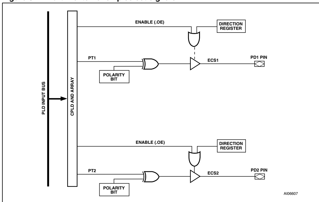
Figure 62. Port D external chip select signals
