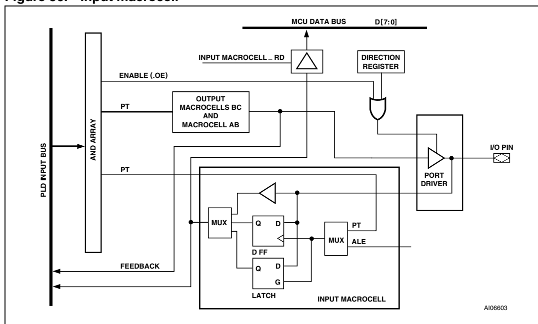
Figure 56. Input macrocell
